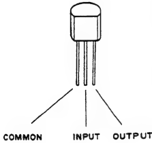
NJM79L ? 7A (JRC) NEGATIVE VOLTAGE REGULATOR (100mA) — FRONT VIEW —
